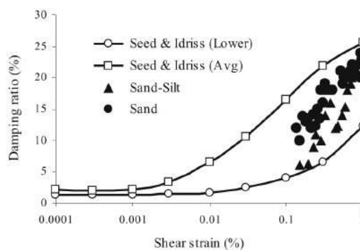
Figure 3. Damping ratio versus shear strain for soils of different fine contents [19]
