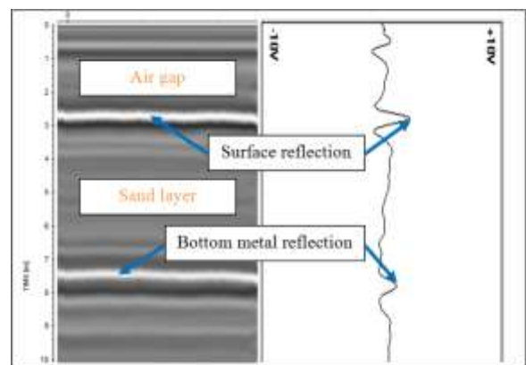
Figure 6. Recorded GPR data for known depth method use
