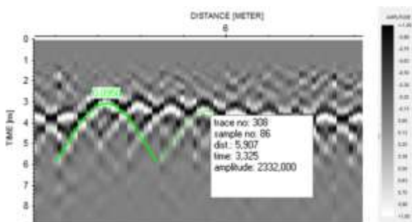
Figure 5. Hyperbolic reflections of steel mesh in concrete floor
