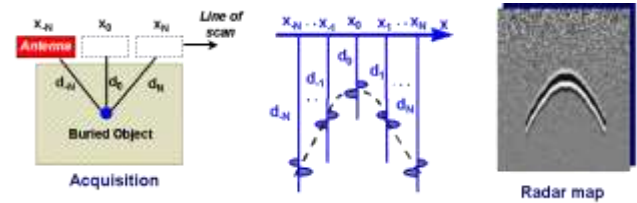
Figure 2. Hyperbolic reflection principle [5]
